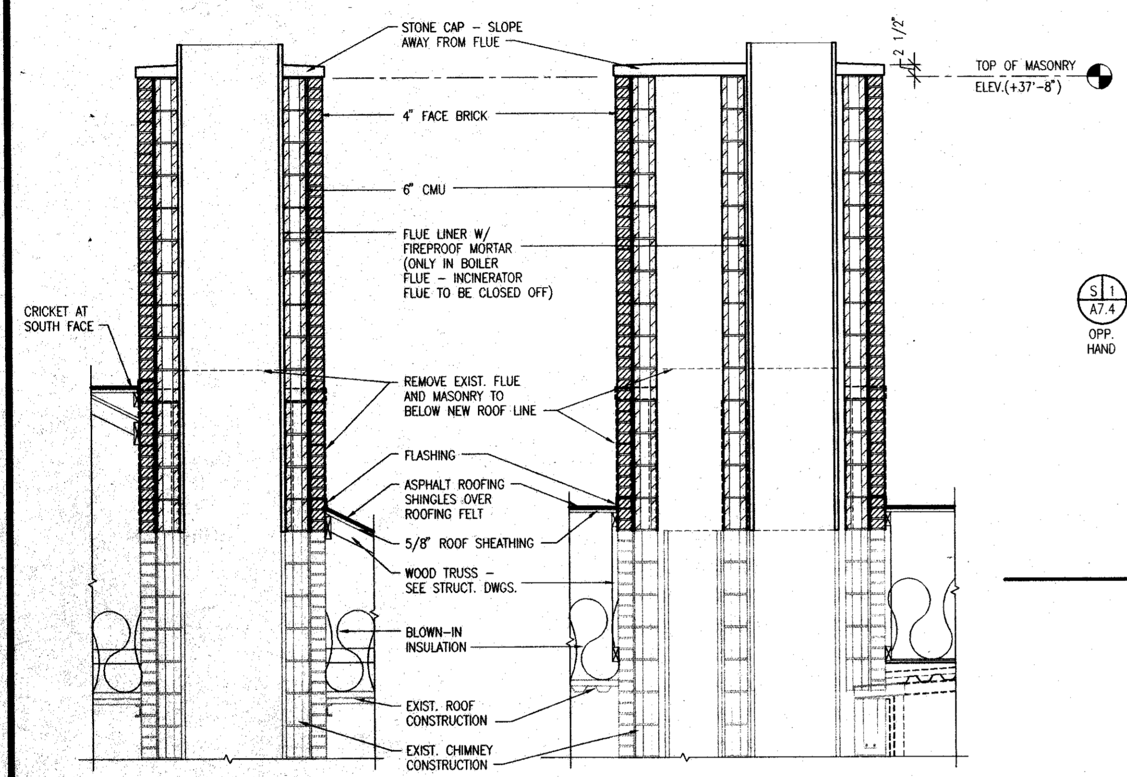
CHIMNEY DETAIL (D13) (A4.1) SCALE: 1/2" = 1'-0"
