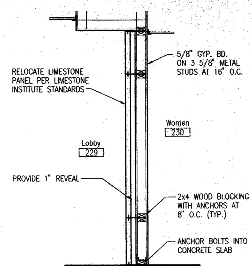
LIMESTONE PANEL DETAIL (D17) (A4.1) SCALE: 1/2" = 1'-0"
