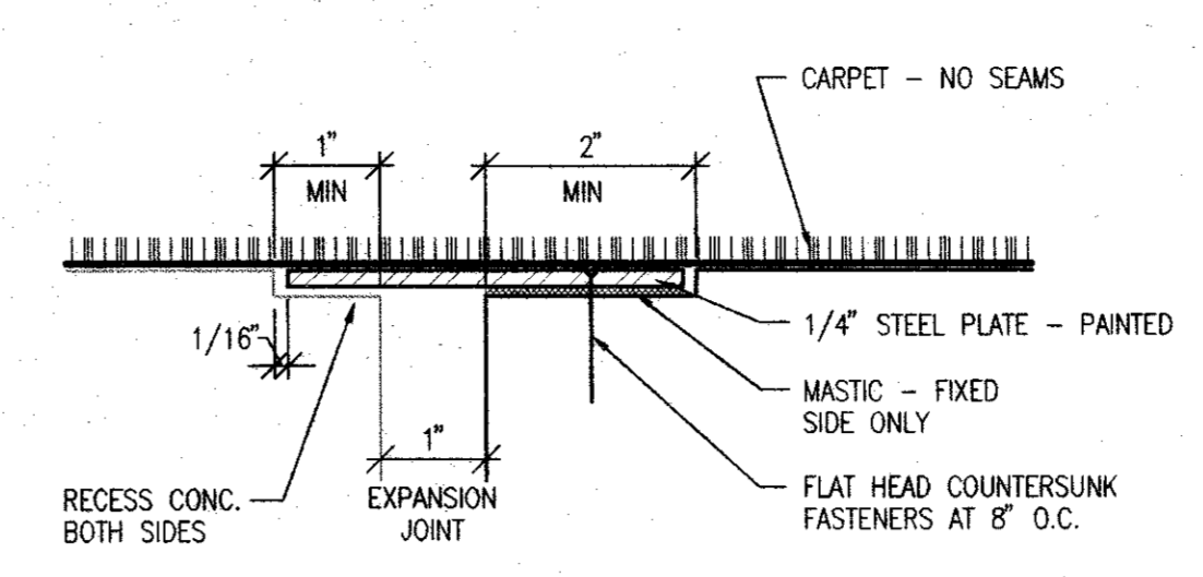
EXPANSION JOINT DETAIL (D15) (A4.1) SCALE: 3" = 1'-0"
