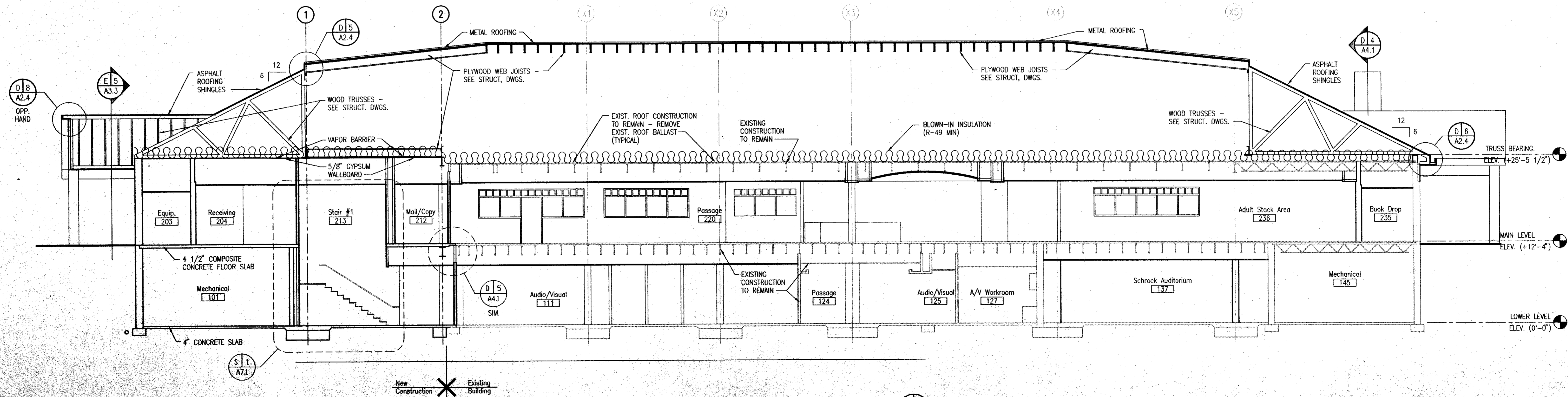
BUILDING SECTION (S2) (A4.1) SCALE: 1/8" = 1'-0"
