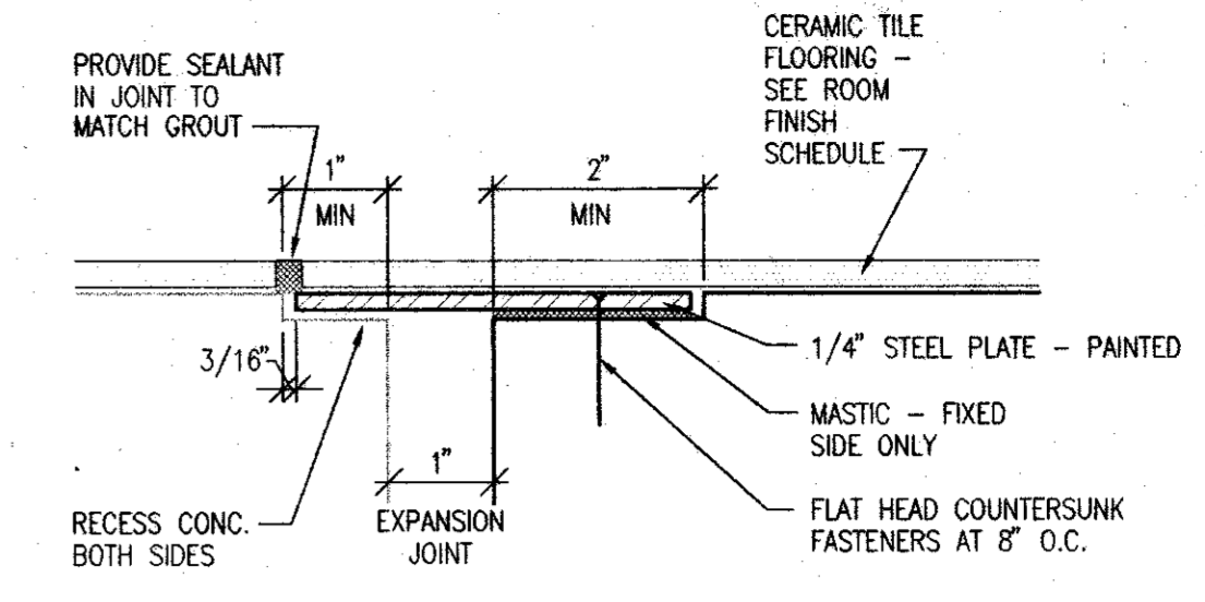
EXPANSION JOINT DETAIL (D16) (A4.1) SCALE: 3" = 1'-0"
