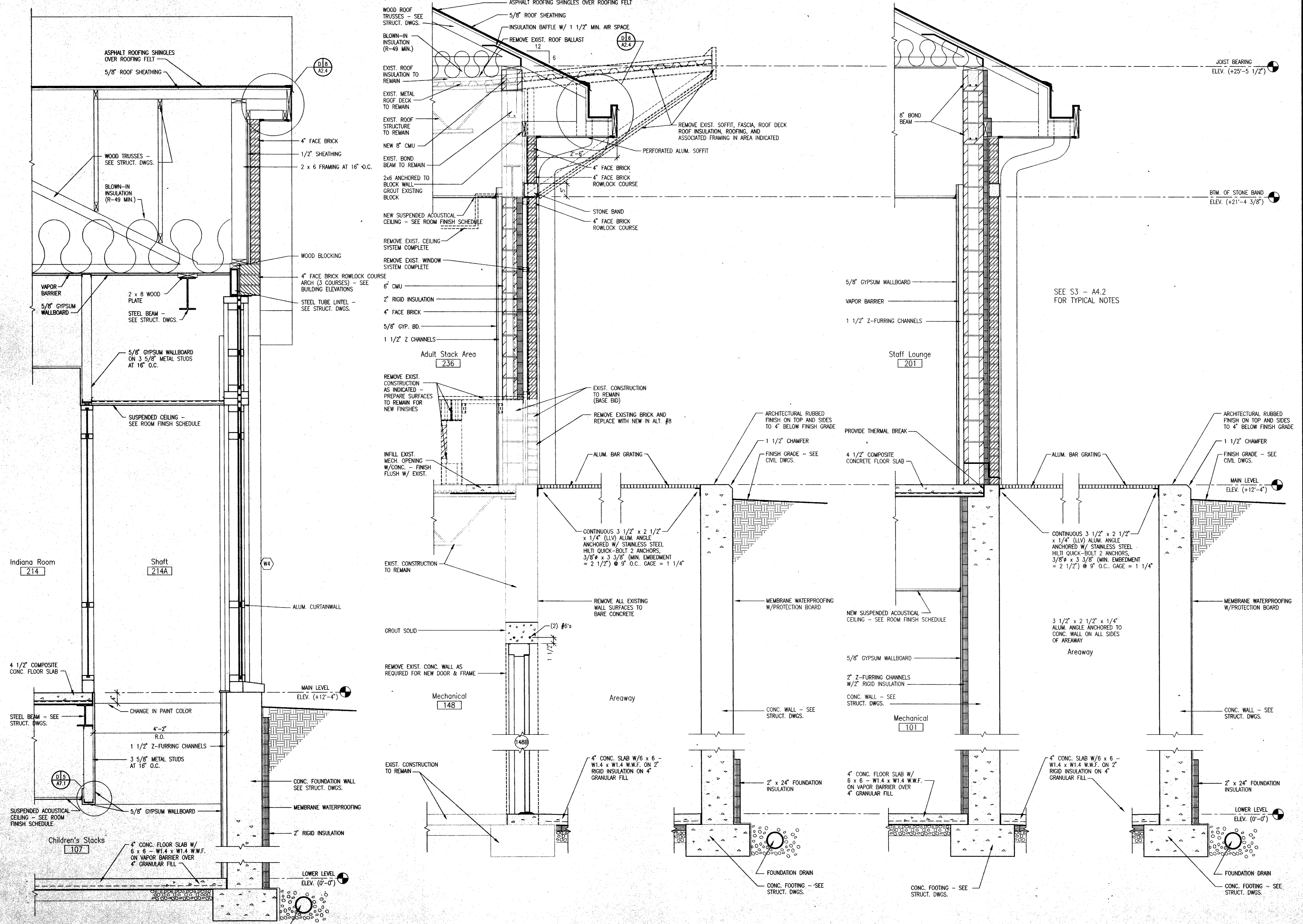
WALL SECTION S3 SCALE: 3/4" = 1'-0" A4.3
