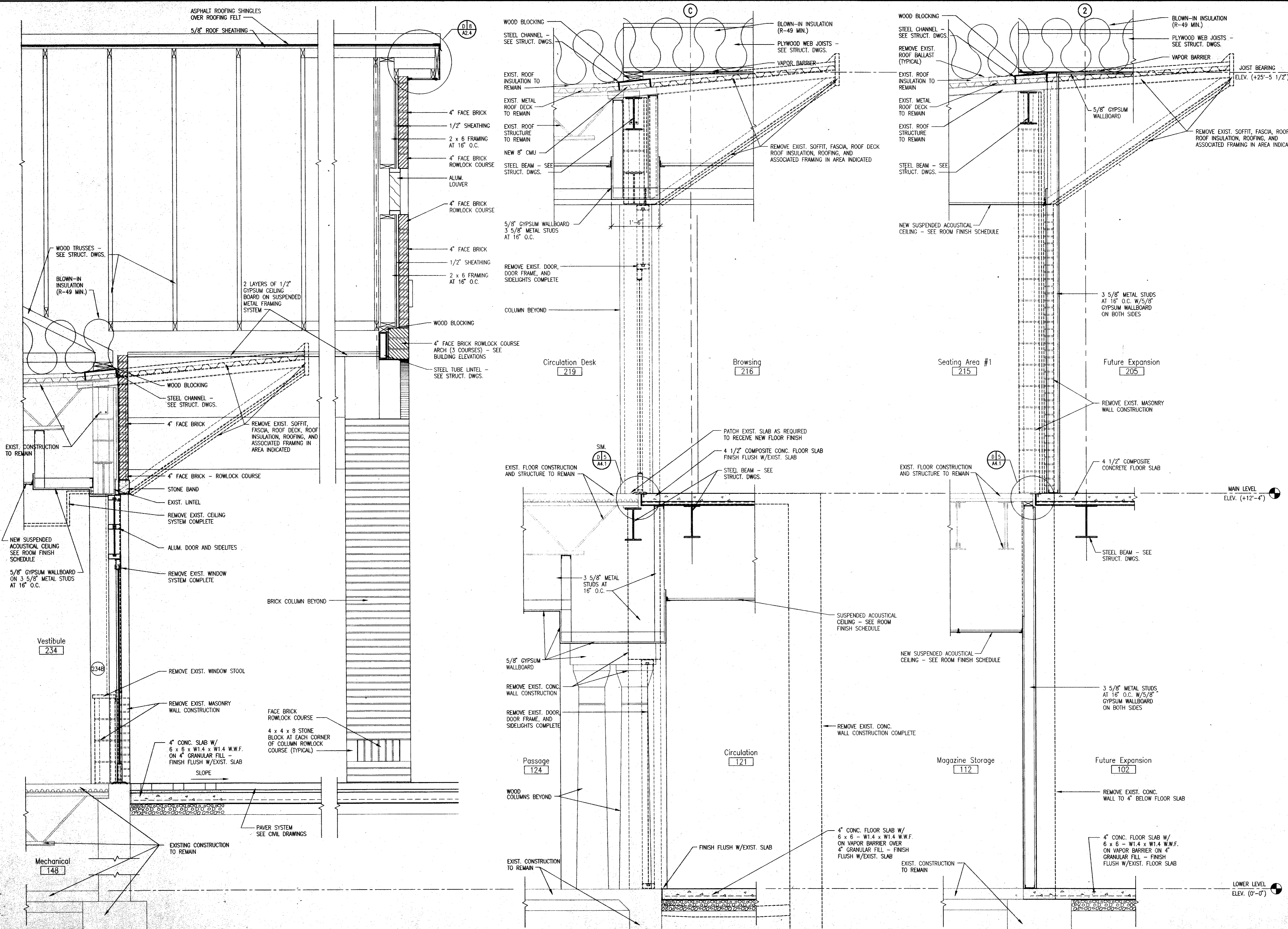
WALL SECTION SCALE: 3/4" = 1'-0"
